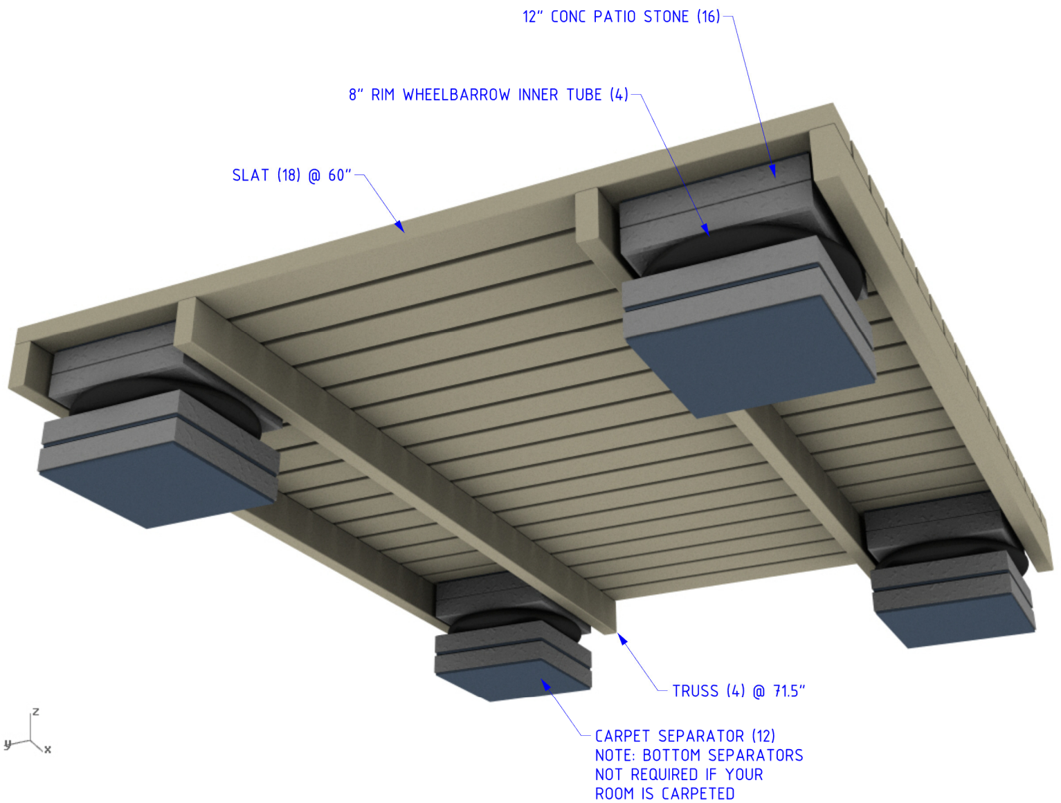
1 UNDERSIDE VIEW JP4 SCALE: NTS
