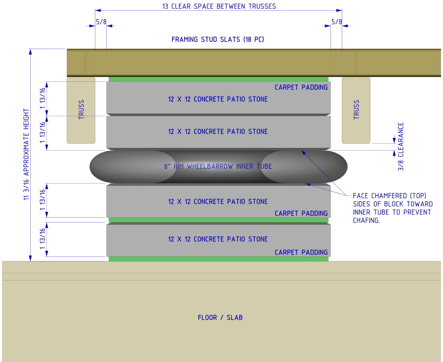
1 ISOLATION PEDESTAL STACK (TYPICAL 4) JP2 SCALE: 1"=3" (1:3)
