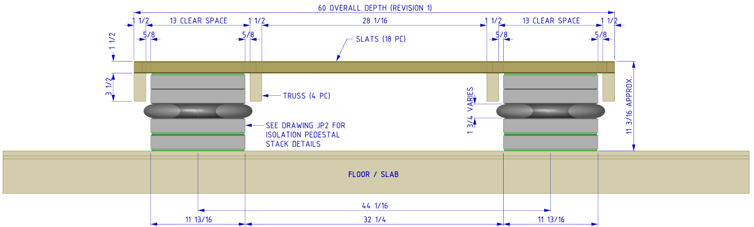
2 SIDE ELEVATION JP1 SCALE: 1"=1' (1:12)
